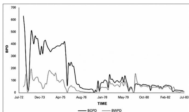
Figure 1. Production Graph of Old Oil Fields
